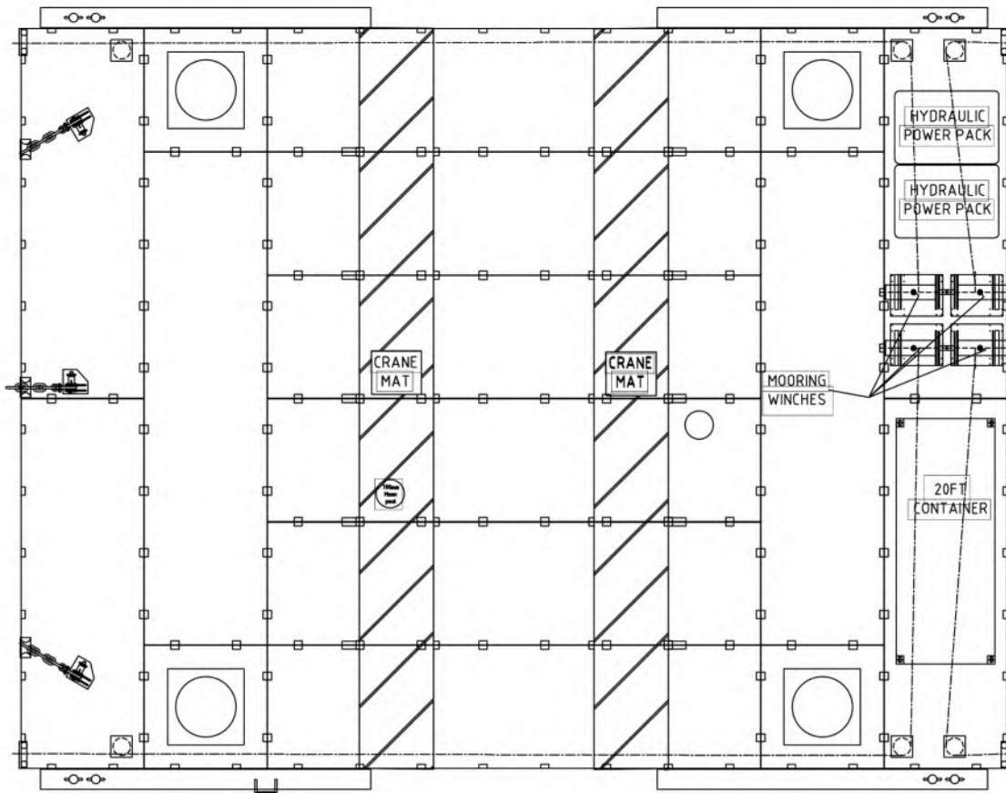
GENERAL ARRANGEMENT
